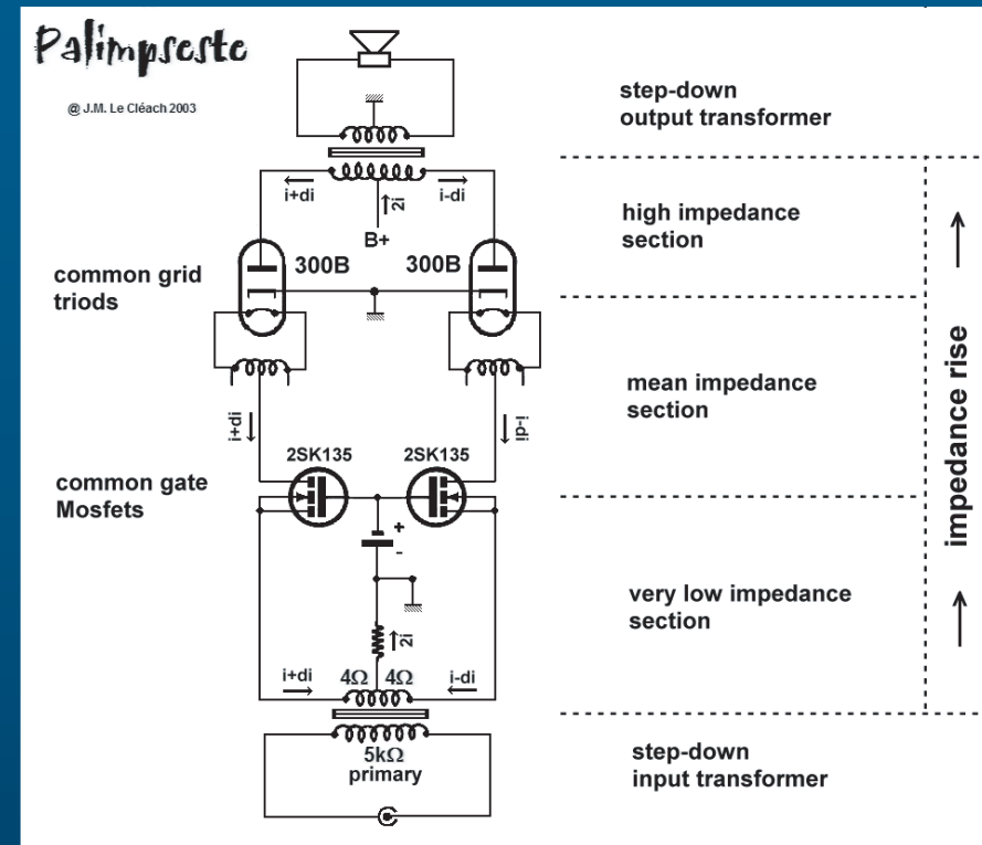
The "Palimpseste" monophonic amplifier
